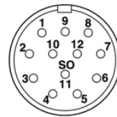
Pin assignment for female plug with external thread, 17-pin View of connection side
