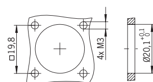
Installation dimensions
