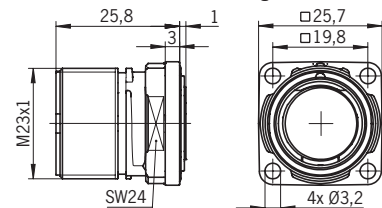
Dimension drawing
